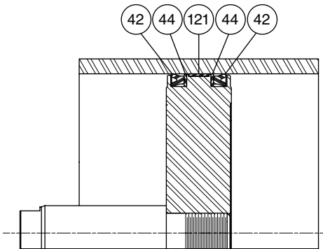
Lipseal Piston with Wear Ring 8" Bore
